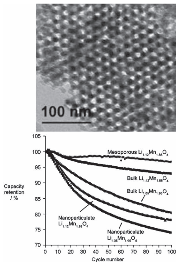
Figure 3. Change in capacity with charge/discharge cycles at 30 mA g -1 (0.3 C) between 3 V and 4.3 V at 50 °C: for mesoporous and bulk Li 1.12 Mn 1.88 O 4 ; bulk and nanoparticulate Li 1.05 Mn 1.95 O 4 ; nanoparticulate Li 1.12 Mn 1.88 O 4 . A TEM image of mesoporous Li 1.12 Mn 1.88 O 4 after 30 cycles was included. Reproduced with permission. [52] Copyright 2008, Wiley-VCH.
